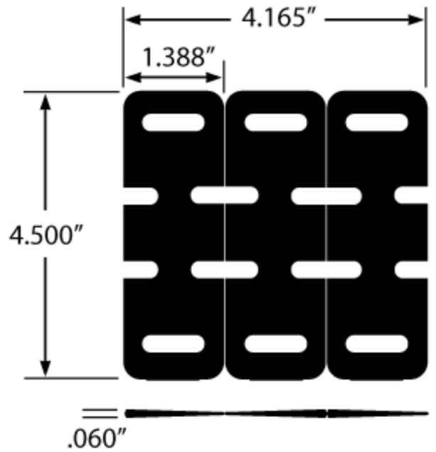
HS 450 BP 4½" QUICK ALIGN HINGE SHIM
