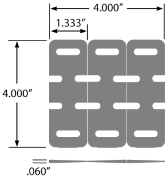
HS 400 BP 4" QUICK ALIGN HINGE SHIM
